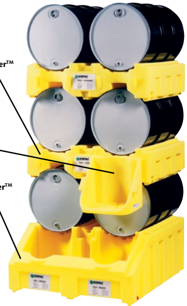
Multi-Purpose Racker/Stacker™
